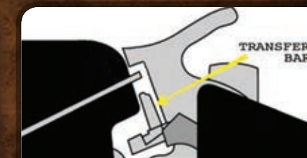
TRANSFER BAR Prevents hammer from striking firing pin unless the trigger is pulled fully to the rear.
